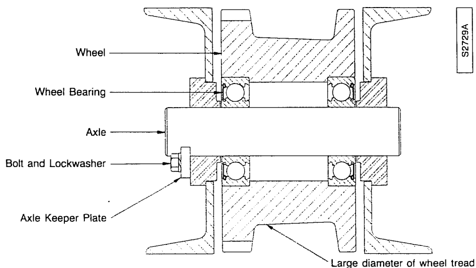
END TRUCK CROSS SECTION
